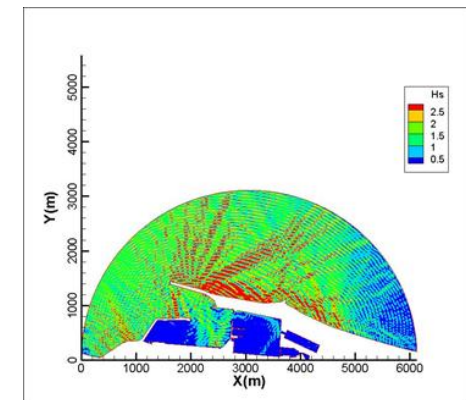
Chennai Port Simulation using FEMSEM
