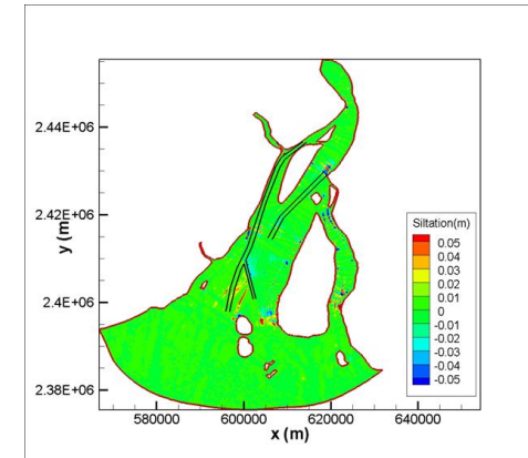
Hoogly River simulation using OCIRC
